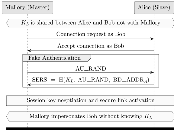
Figure 3: Authentication spoofing on Bluetooth Legacy Authentication process. Mallory establishes a connection with Alice while impersonating Bob. Mallory sends AU_RANDOM to Alice and receives SERS from Alice. Since the Bluetooth Specification does not require mutual authentication, Alice does not have to verify that Mallory knows K_L .
