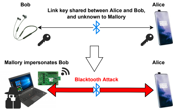
Figure 1: Blacktooth attack overview: Alice and Bob share a link key that is unknown to Mallory. Mallory's goal is to establish a Bluetooth connection with Alice and get the privilege through sensitive profiles while impersonating Bob. The attack is utterly stealthy without the victim's interactions.
