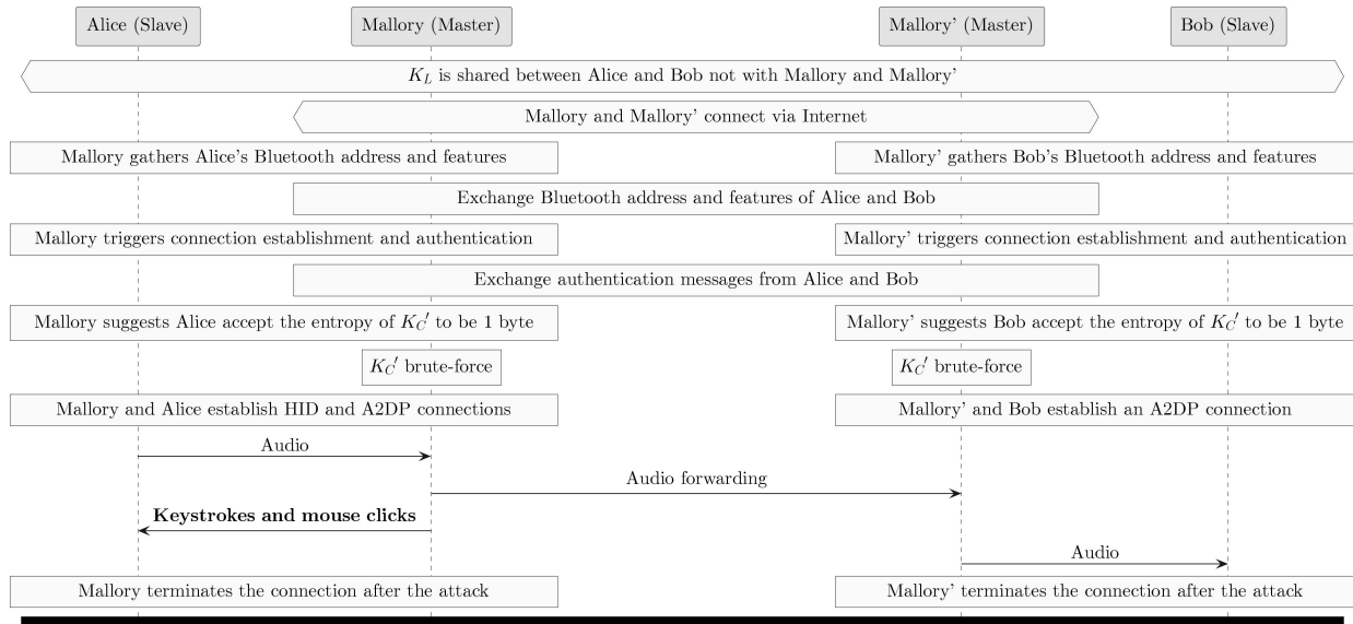
Figure 6: Stages of the MITM Blacktooth attack.
