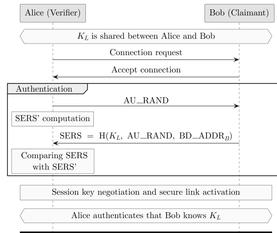
Figure 8: Legacy Authentication process. The legacy Authentication process authenticates devices unilaterally. To achieve mutual authentication, the authentication process should be completed by Alice and Bob respectively.
