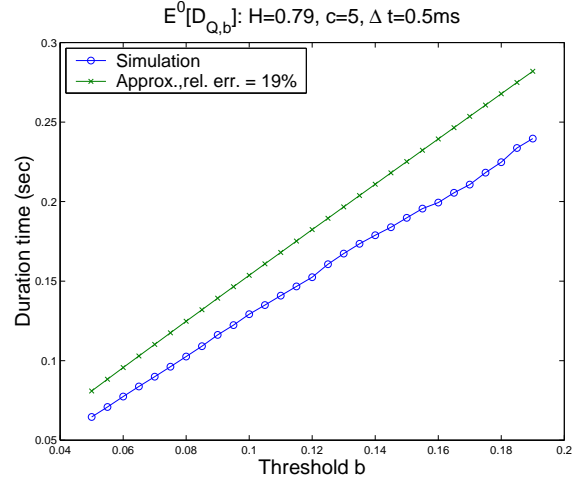
(b) Duration of busy periods vs b
