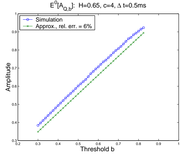
(a) Amplitude vs b
