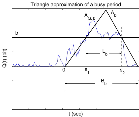
Fig. 4. Triangle approximation of a busy period
