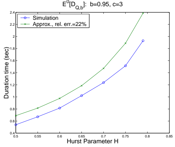
(b) Duration of busy periods vs H
