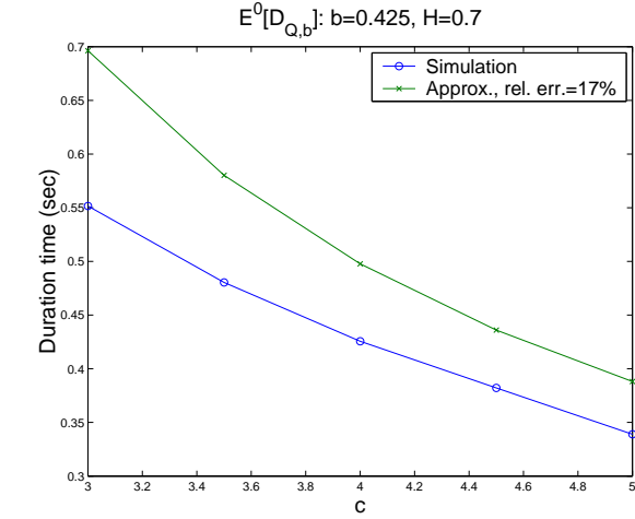
(a) Duration of busy periods vs c
