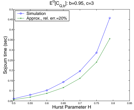
(b) Sojourn time vs H
