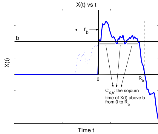
(b) Approximation process X(t)
