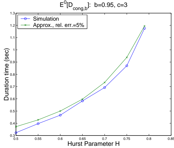
(b) Duration of congestions vs H
