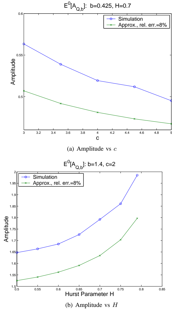
Fig. 14. Comparison of mean amplitude of congestion events
