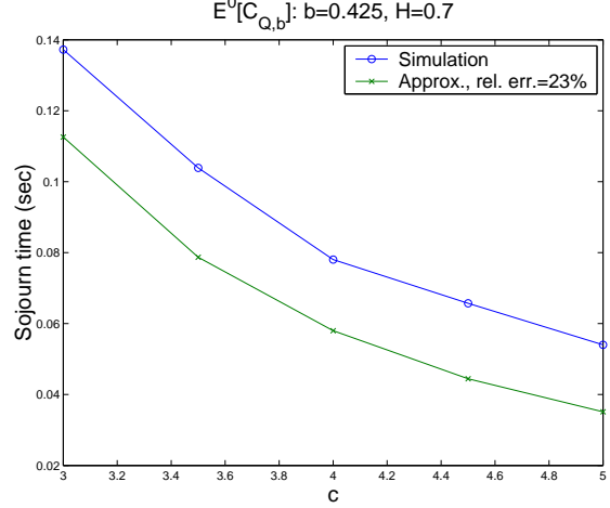
(a) Sojourn time vs c
