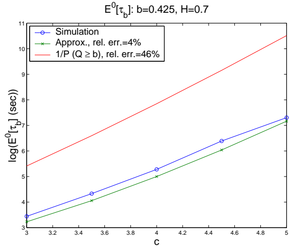
(a) Inter-congestion time vs c
