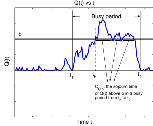
(a) A busy period of Q(t)
