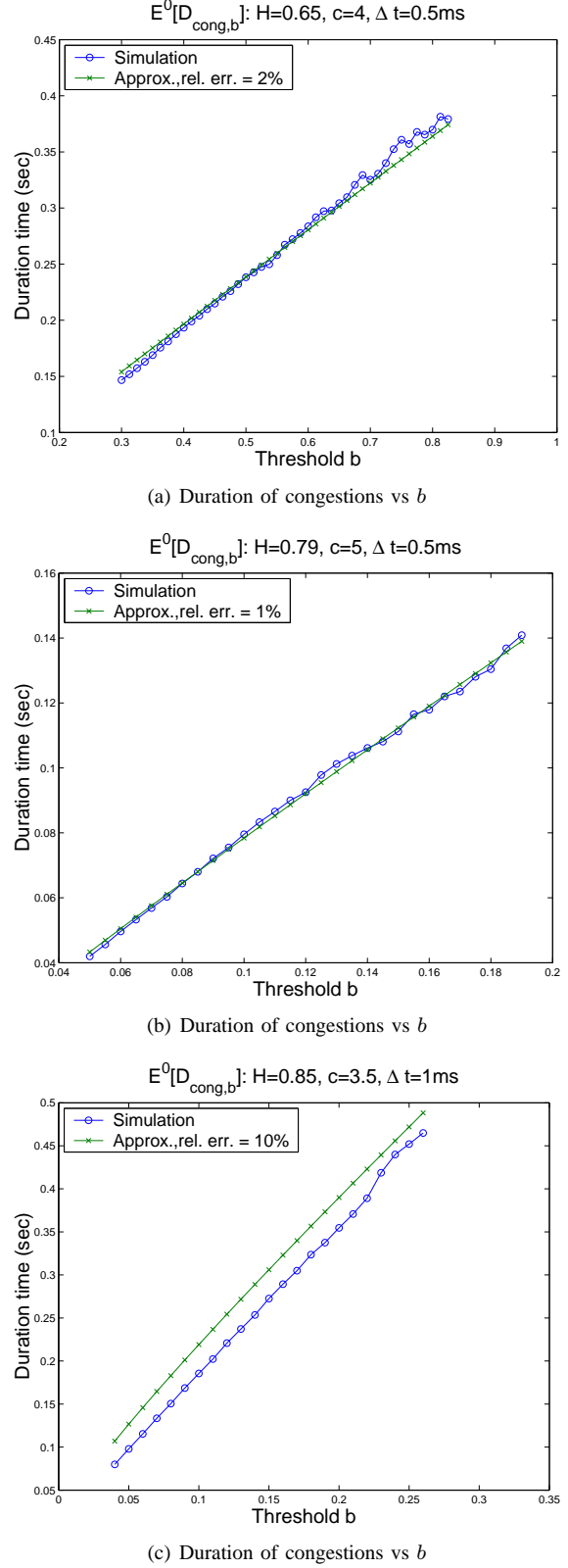
Fig. 9. Comparison of mean duration of congestion events
