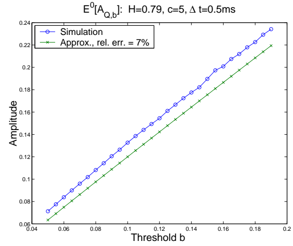
(b) Amplitude vs b
