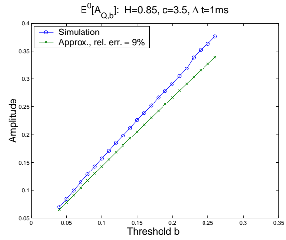
(c) Amplitude vs b
