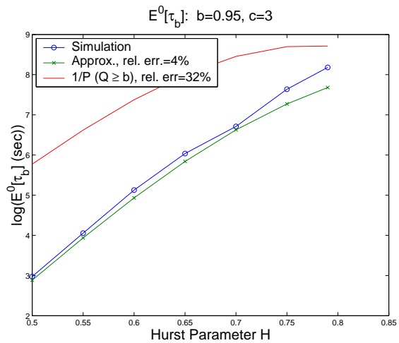
(c) Inter-congestion time vs H
