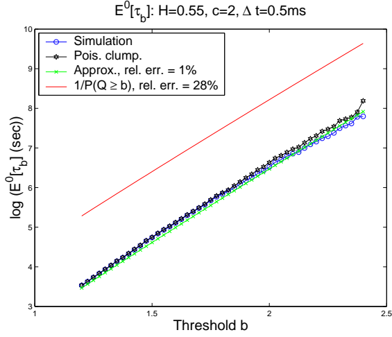
(a) Inter-congestion time vs b
