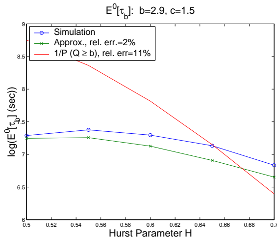
(b) Inter-congestion time vs H
