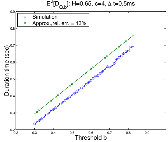
(a) Duration of busy periods vs b
