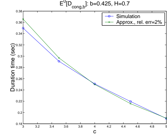
(a) Duration of congestions vs c
