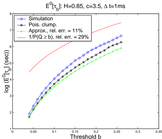
(c) Inter-congestion time vs b
