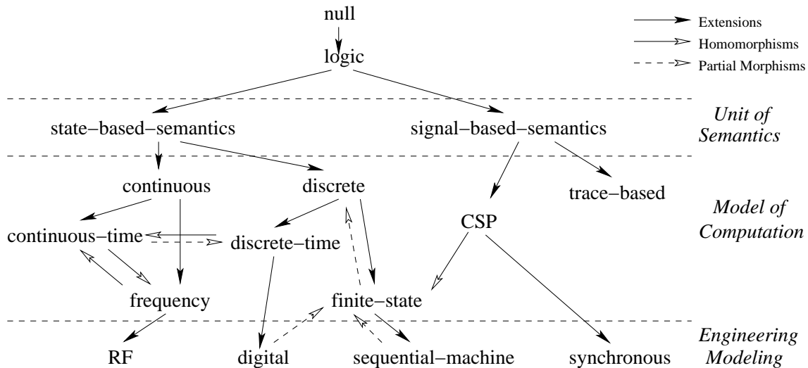
Figure 6.1: Lattice of pre-defined specification domains.
