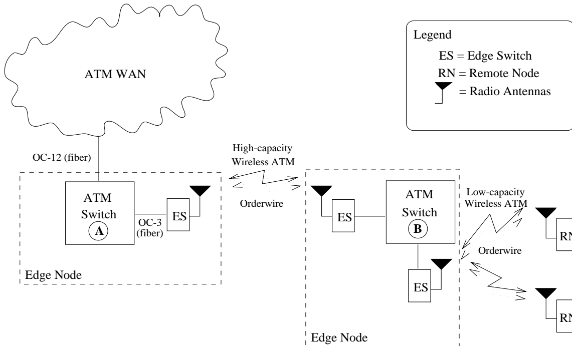
Figure 1. RDRN High-level Architecture.
