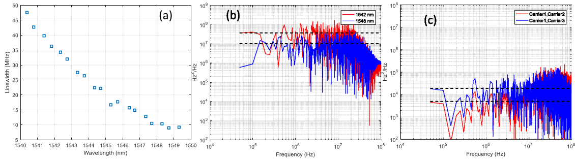
Fig. 2. (a) Optical linewidth as a function of wavelength obtained from the setup shown in Fig. 1. (b) the FM noise spectrum of the comb line in the vicinity of 1542 nm and 1548 nm. (c) FM noise spectrum of differential phase noise between carrier 1 and carrier 2 (red); carrier 1 and carrier 3 (blue).
