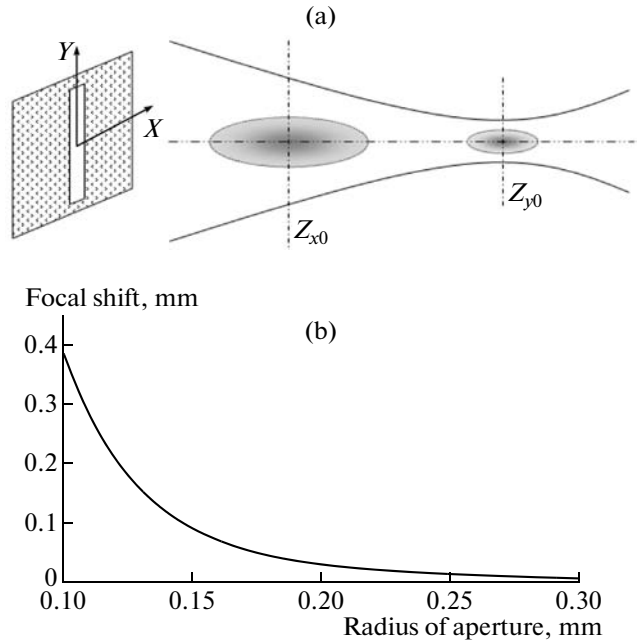
Fig. 1. Focal positions of a focused Gaussian beam after a slit (a). Due to Fresnel numbers are different for two orthogonal directions, focal shift at x direction is more bigger than y direction. As a results, the real focus of focused Gaussian beam after slit will locate between Z_{x0} and Z_{y0} . (b) Shows the dependence of focal shift on radius of aperture.
