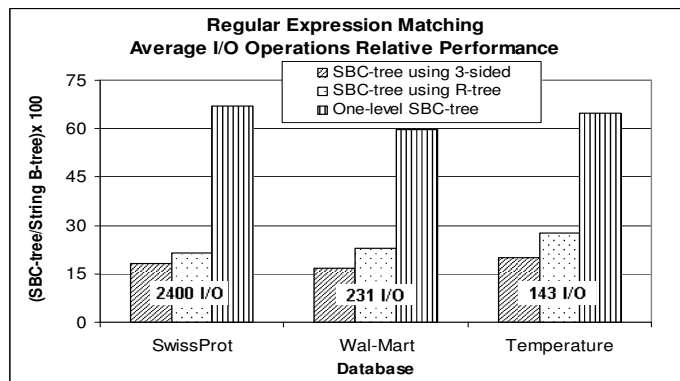
Figure 12: The regular expression queries
