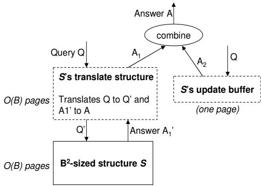
Figure 6: Query processing over the 3-sided structure
