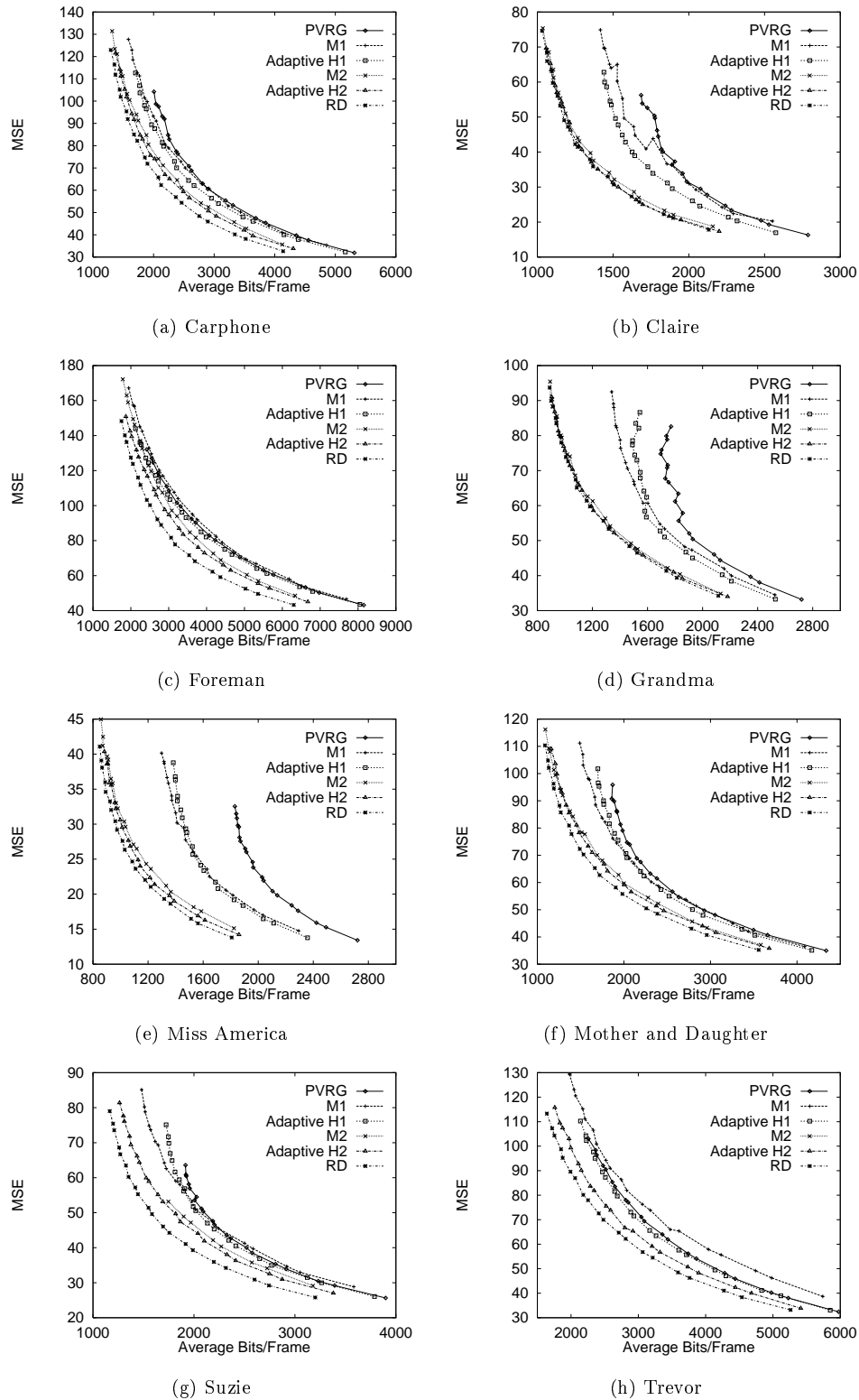
Fig. 11. Performance of motion estimation algorithms on eight test sequences.
