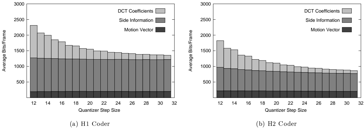
Fig. 12. Distribution of bits for coding the Miss America sequence with the adaptive heuristic coder.
