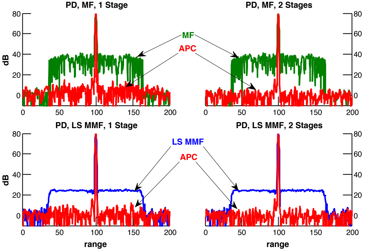
Figure 3.14: Matched filter, LS MMF and APC responses for PD in a two-target environment with worst-case straddling. The top two plots show the responses of the matched filter and APC initialized with the matched filter. The bottom two plots show the responses of the LS MMF and APC initialized with the LS MMF. Neither the matched filter nor the LS MMF can discern the smaller target. The smaller target can be found after one adaptive stage for both the matched filter and LS MMF initializations.
