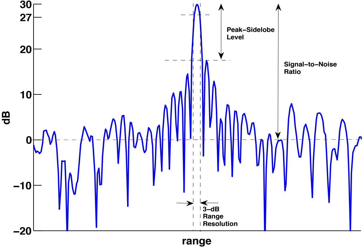
Figure 1.1: Visual representation of range response PSL, 3 dB range resolution, and SNR.
