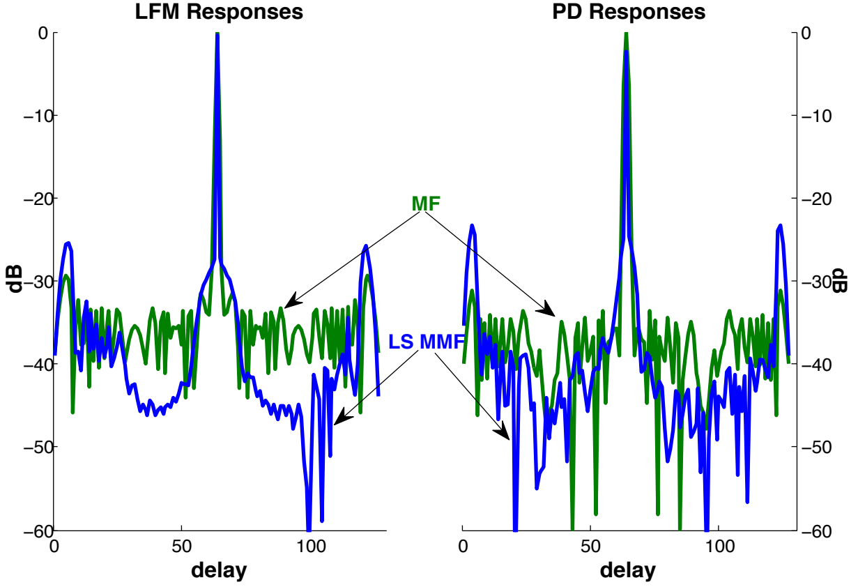
Figure 2.2: Matched filter and LS MMF responses for LFM and PD with K = 1 , M = 1 , and BT = 64 . The matched filter outperforms the LS MMF in terms of MML and PSL, while the LS MMF has lower sidelobe levels near the mainlobe, with an increase near the ends of the filter response.
