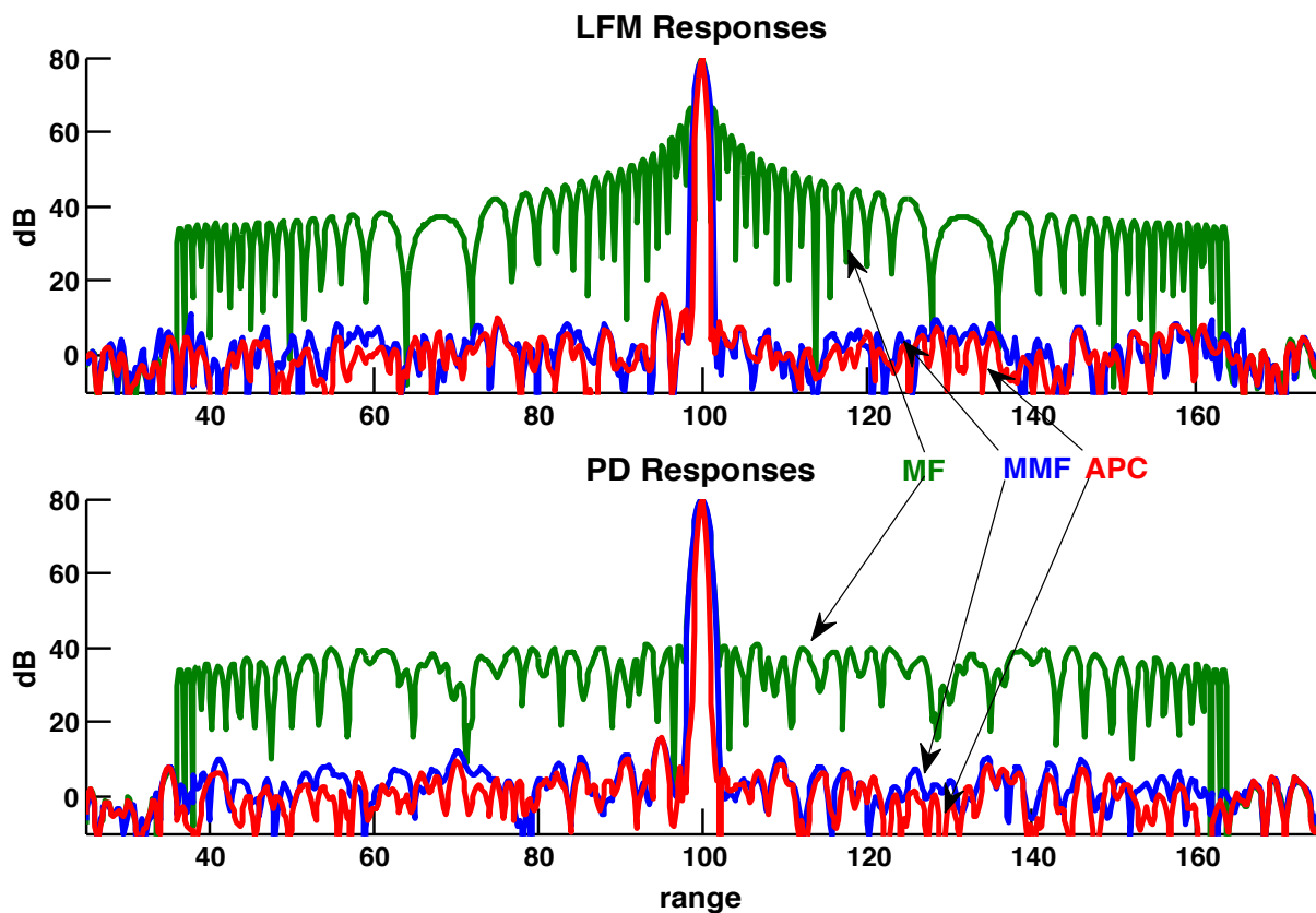
Figure 3.20: Matched filter, LS MMF and APC responses for LFM and PD in a two-target environment. The larger target has a Doppler shift of 0.04 radians, while the smaller target has no Doppler shift. The LS MMF was used to initialize APC. For both waveforms, the LS MMF and APC are able to discern the smaller target, and APC further suppresses sidelobes below the levels in the LS MMF response.
