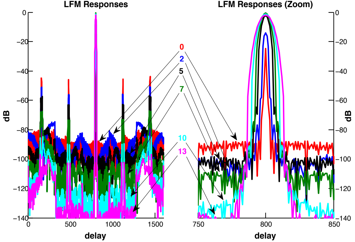
Figure 2.7: LS MMF responses for LFM with beamspoiling. The number of rows that were zeroed above and below the m^{th} row of \tilde{\mathbf{A}} , in decreasing order, are 13, 10, 7, 5, 2, and 0. The responses on the right are the zoomed-in mainlobes of the responses on the left. As more rows are zeroed, the mainlobe width increases and surpasses the matched filter mainlobe width. The minimum MML occurs when 7 rows are zeroed.
