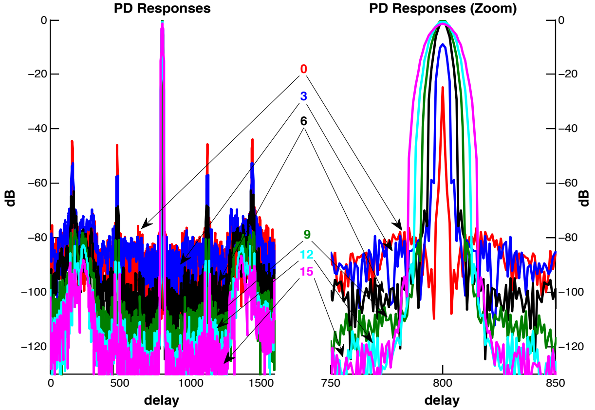
Figure 2.8: LS MMF responses for PD with beamspoiling. The number of rows zeroed above and below the m^{th} row of \tilde{\mathbf{A}} , in decreasing order, are 15, 12, 9, 6, 3, and 0. The responses on the right are the zoomed-in mainlobes of the responses on the left. As more rows are zeroed, the mainlobe width increases and surpasses the matched filter mainlobe width. The minimum MML occurs when 9 rows are zeroed.
