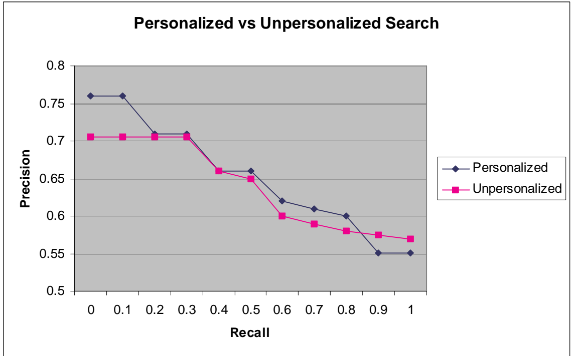
Figure 1. Recall and Precision with and without Personalized Reranking.
