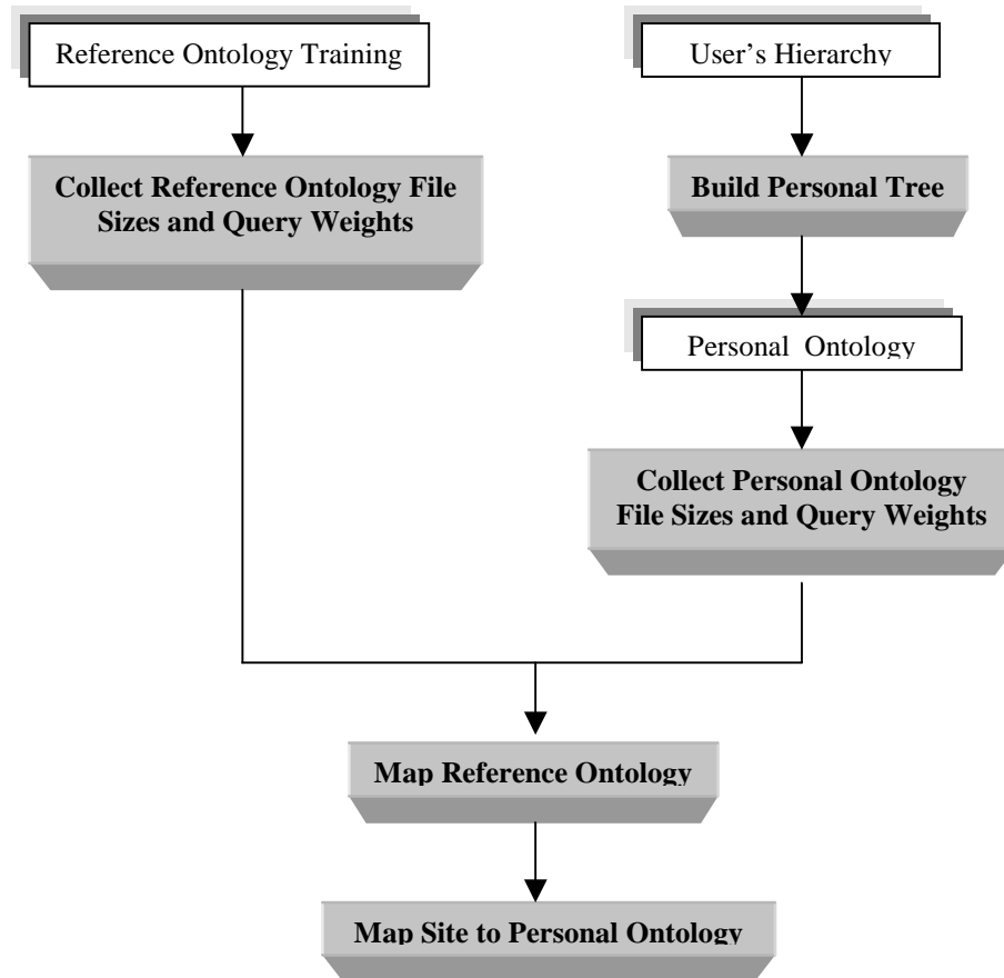
Figure 3. Personalized Browsing Architecture.
