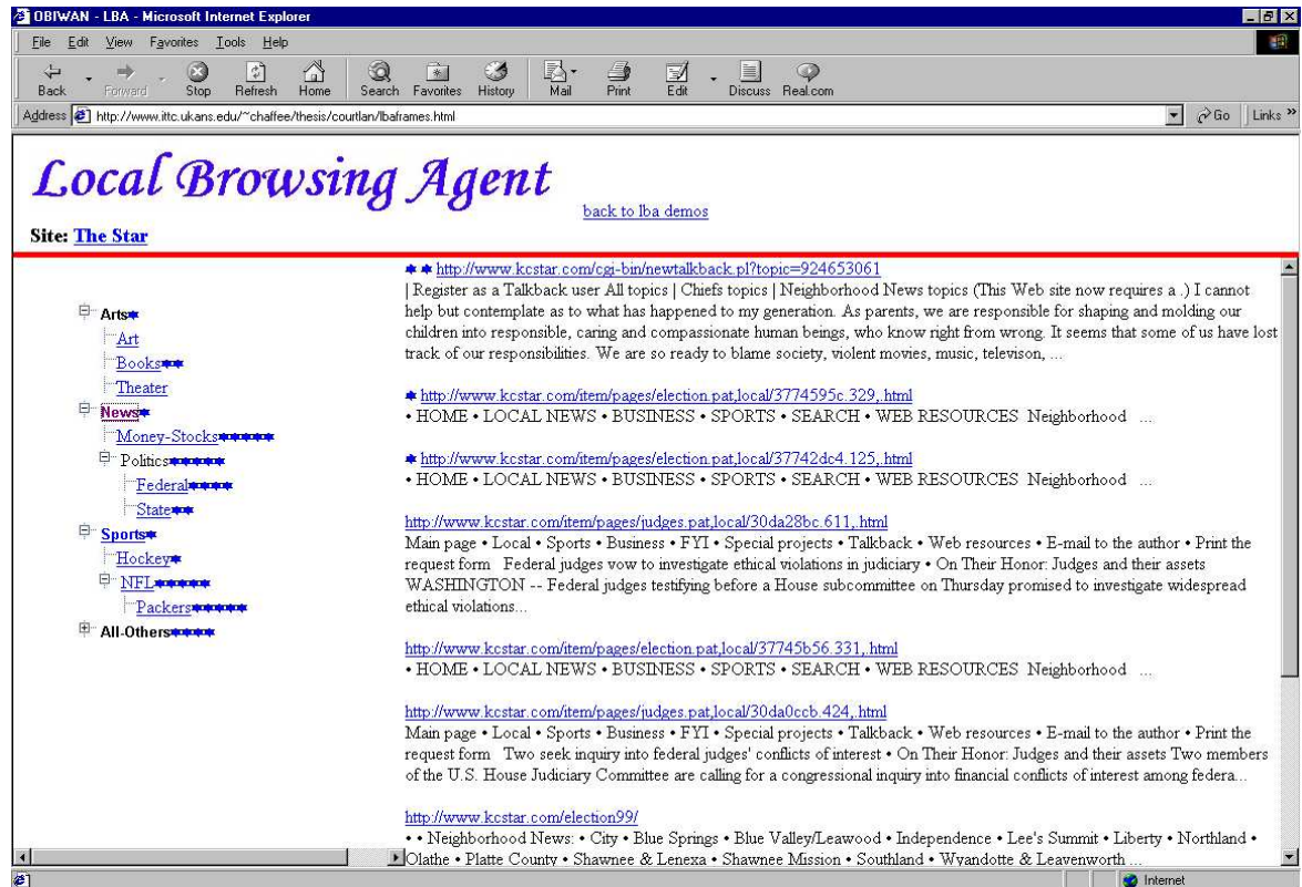
Figure 5. Screen Shot of a Web Site's Content Displayed after being Mapped to the Personal Ontology.
