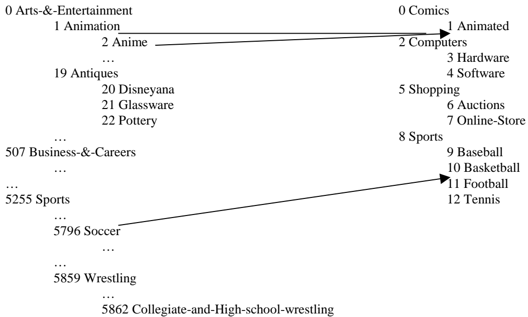
Figure 4. The Reference Ontology Mapped to a Personal Ontology
