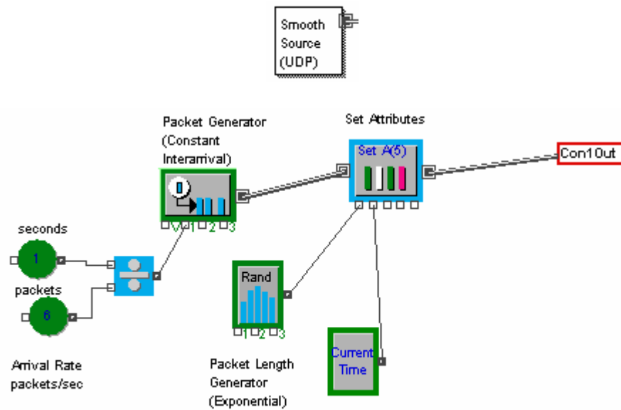
Figure 6: Smooth Source Model Block
