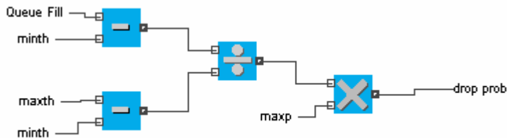
Figure 8: RED Dropping Probability
