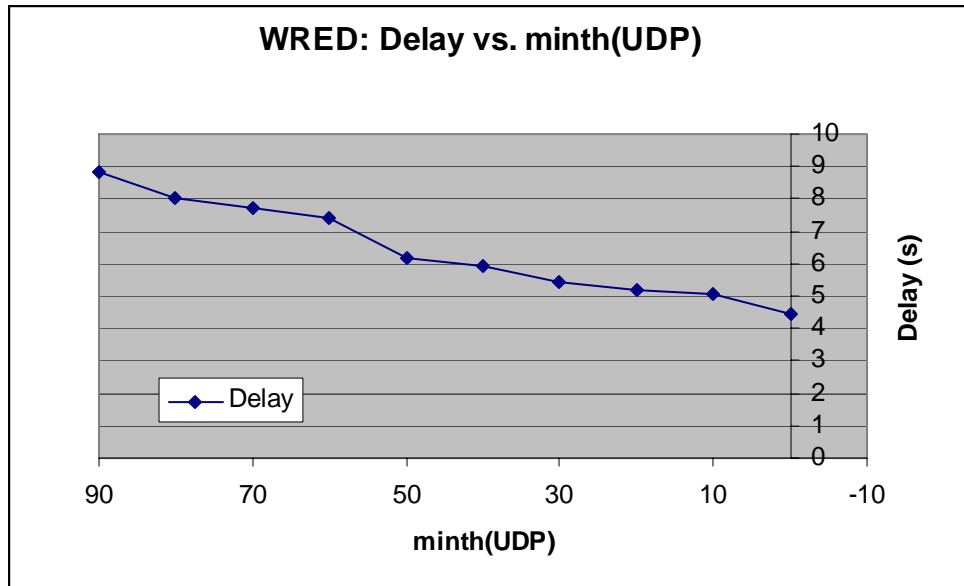
Figure 23: WRED Packet Delay vs. minth(UDP) , \rho=1.2
