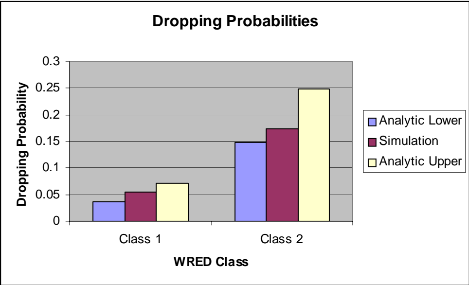
Figure 13: Dropping Probability by WRED Class
